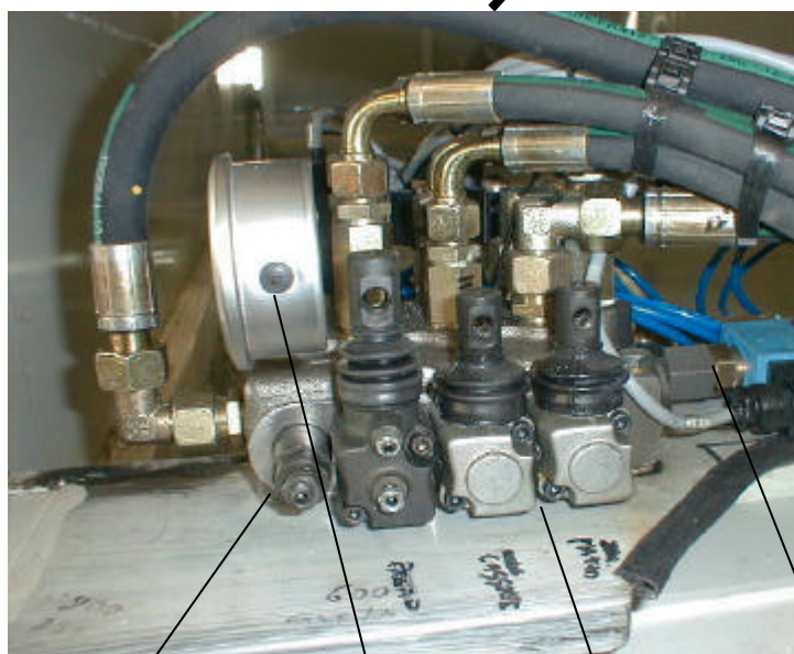
VISTA FRONTE FRONT VIEW
